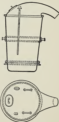
FIG. 13.—Heraeus' Varnish-kettle.
